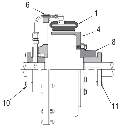
PCB - 205 Arrangement
